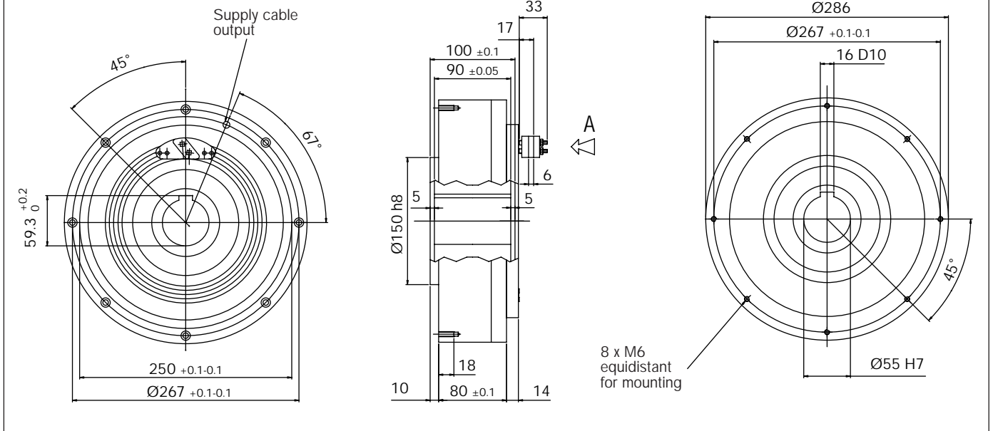
VIEW A - Brushes holder
